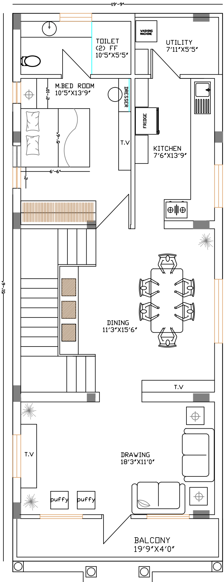
1st FLOOR FURNITURE LAYOUT OF VILLA NO 16
