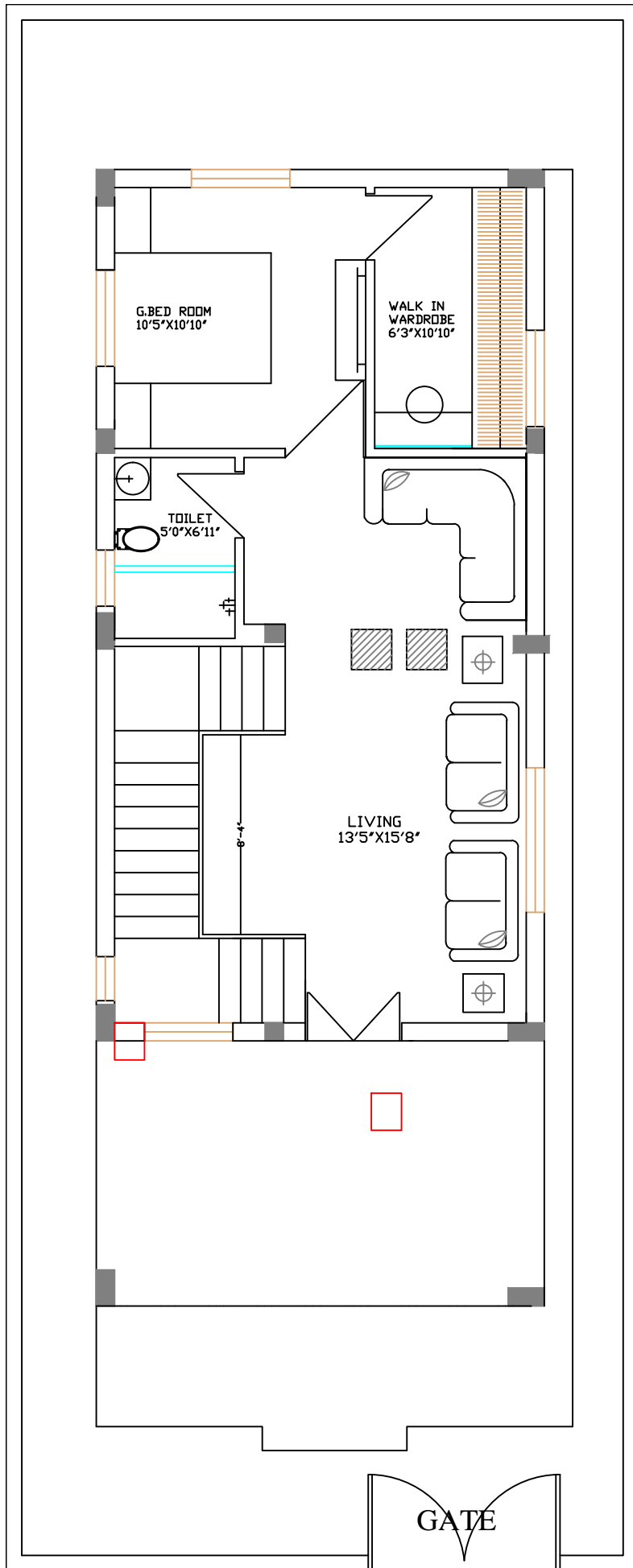
G.FLOOR PLAN OF VILLA NO 16
